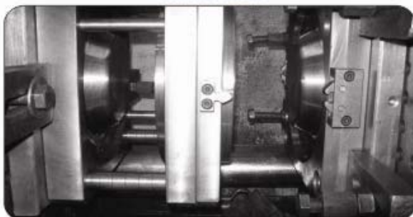
Fully Automatic 2 Cavity Mould for Dish Plate
